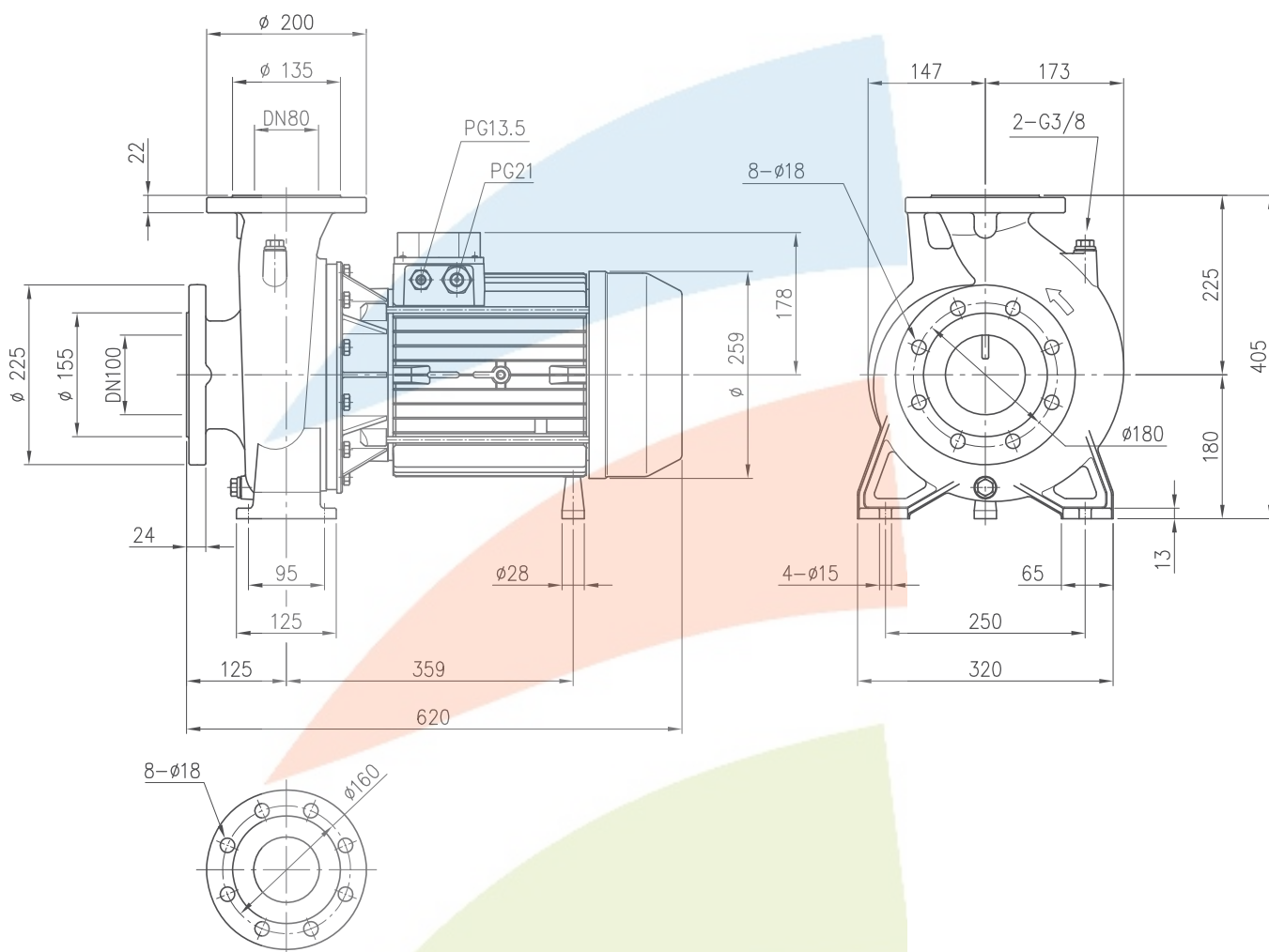
PUMP 3LM 80-160/11
