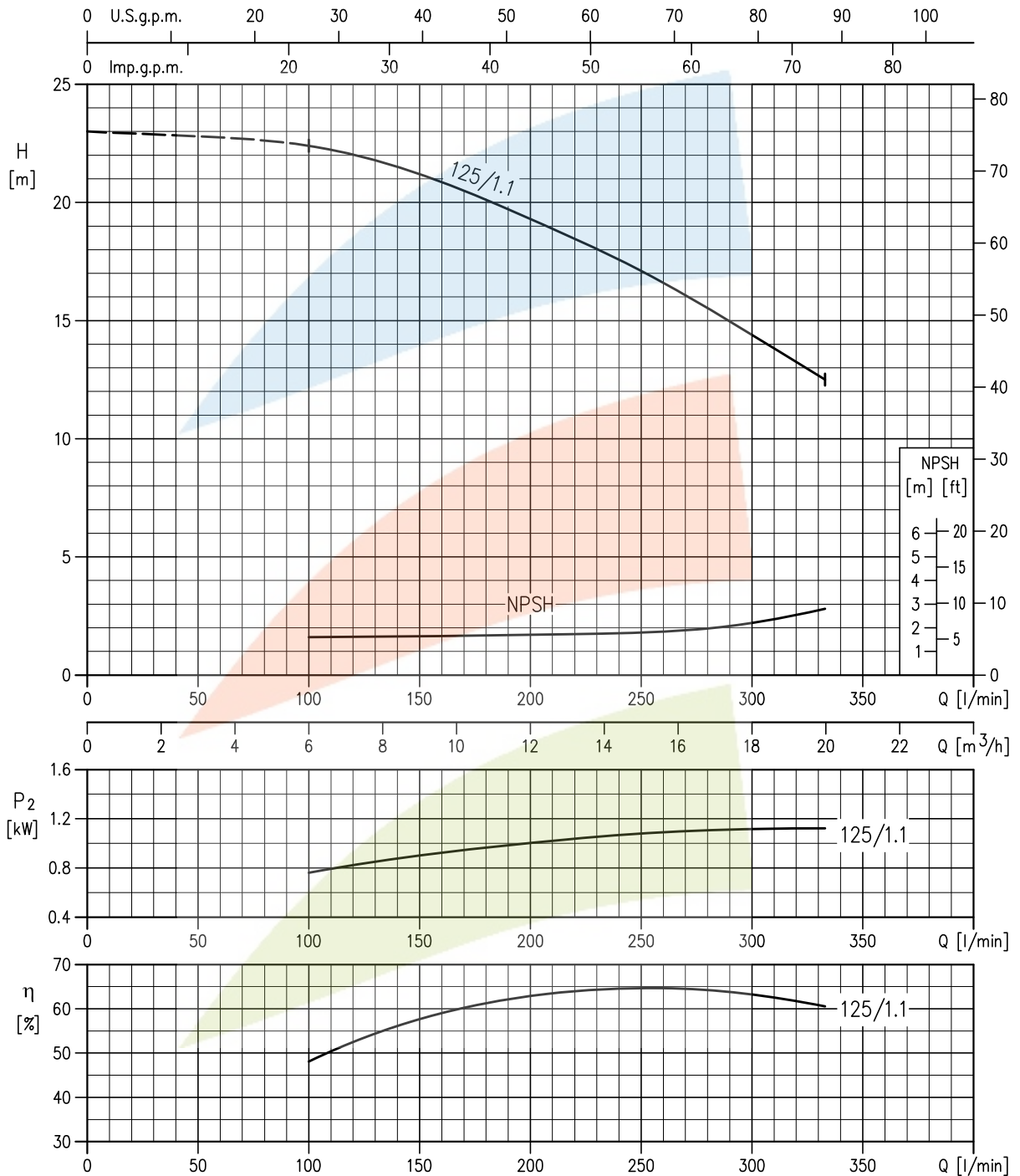
32-125/1.1 (1.1kW) MEI > 0.70 – impeller diameter = 133 mm
