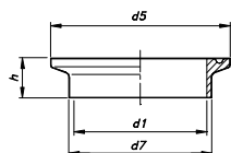
CASQUILLO CL SOLD. CORTO SHORT WELDING CLAMP FERRULE CL SOUDER COURTE.
